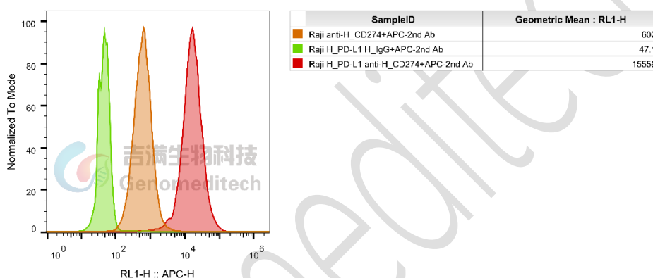
Figure 1 | H_PD-L1 Raji Cell Line (Cat. GM-C03541) was determined by flow cytometry using Anti-H_CD274(PDL1) hIgG1 Antibody(Atezolizumab) (Cat. GM-31740AB ).
